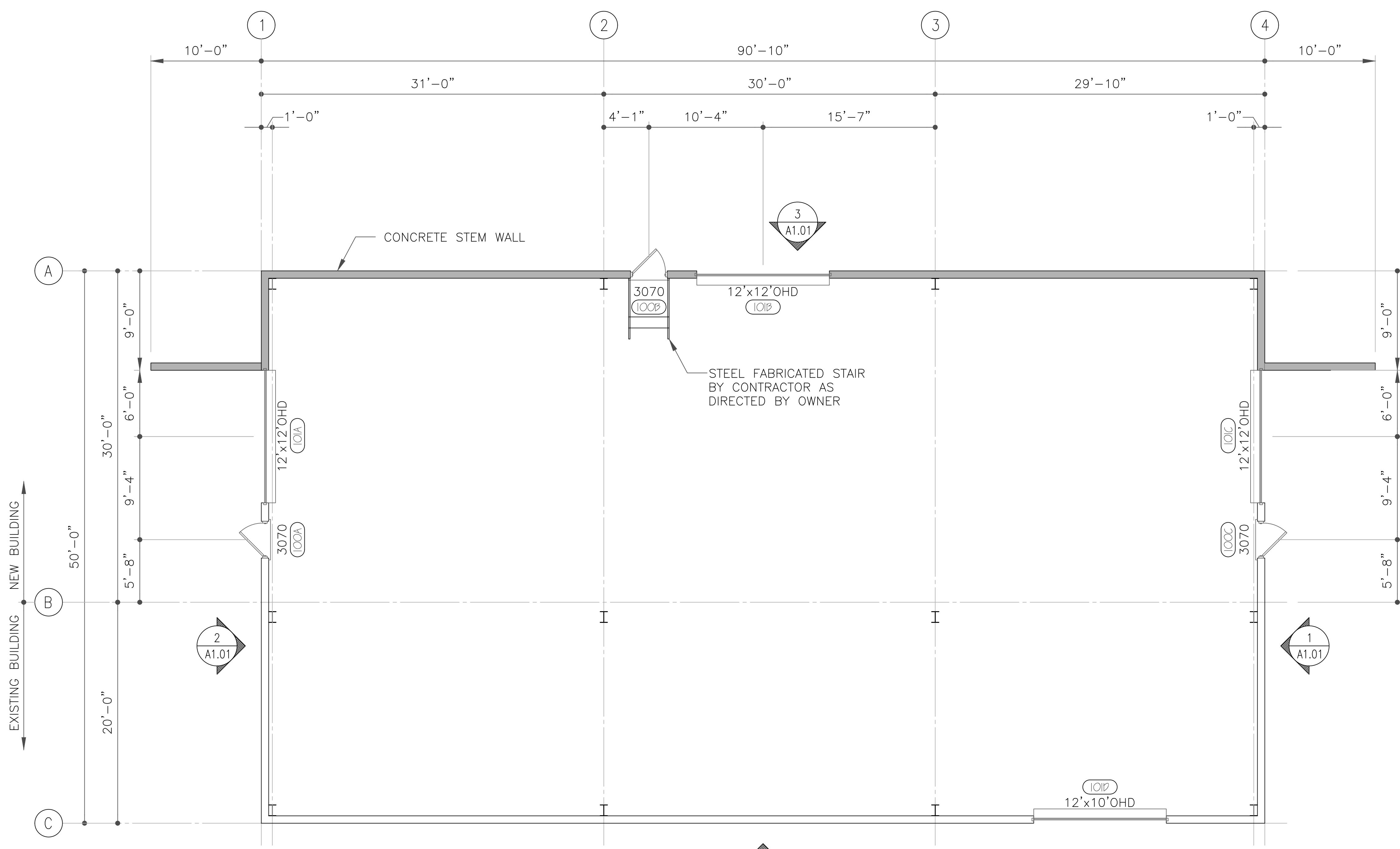
FLOOR PLAN TOP OF CONCRETE AT ELEVATION 100'-0" UNLESS OTHERWISE NOTED BY (+) OR (-). SCALE: 3/16" = 1'-0"
