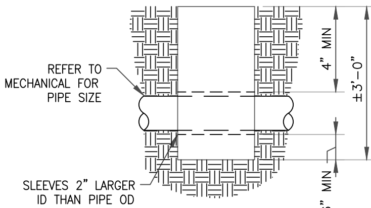
7 TYP PIPE SLEEVE THROUGH GRADE BEAM OR FOOTING
