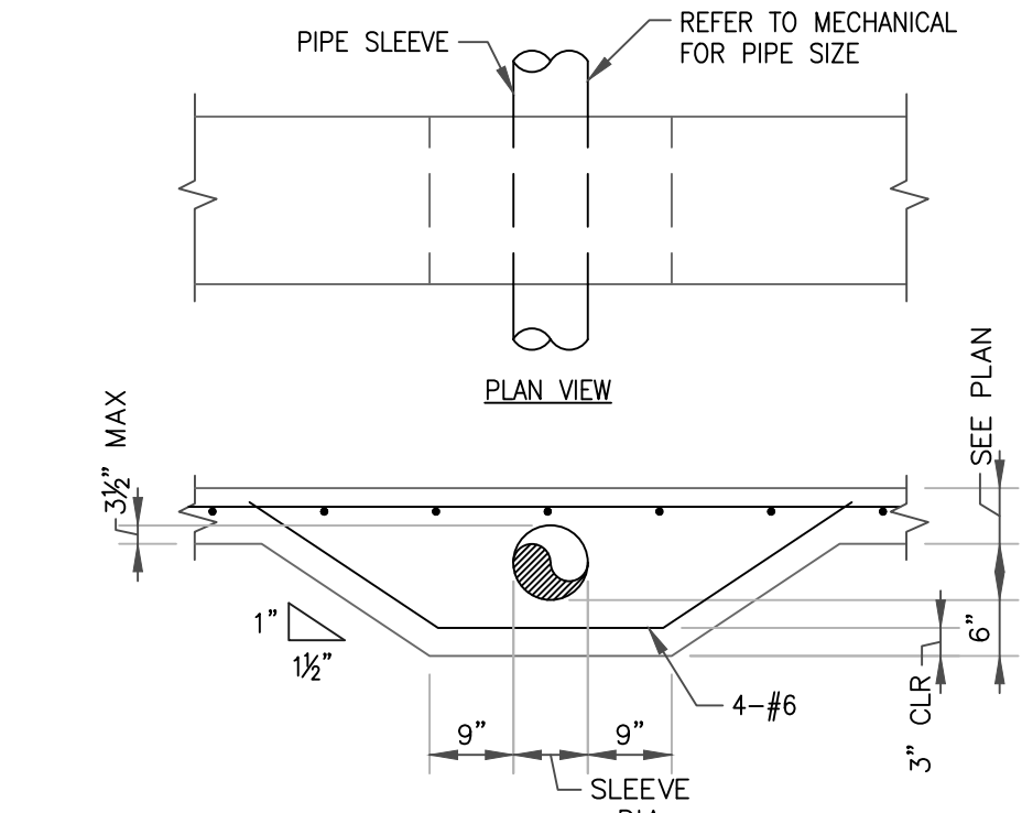
2 TYP DEEPENED BEAM @ PIPE SLEEVE
