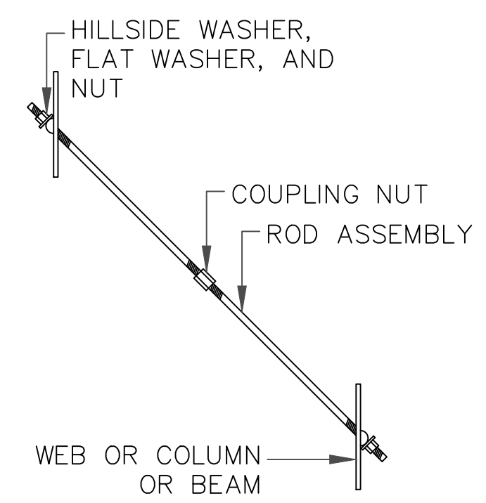
2 CONNECTION TO EXISTING STRUCTURE
