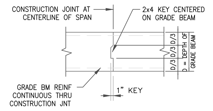
4 TYP GRADE BEAM CONSTRUCTION JOINT
