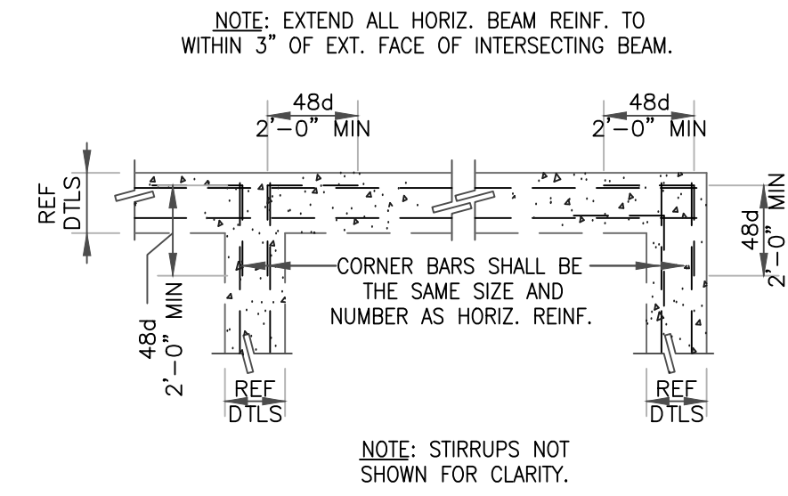
9 TYP GRADE BEAM CORNER BAR REINF.
