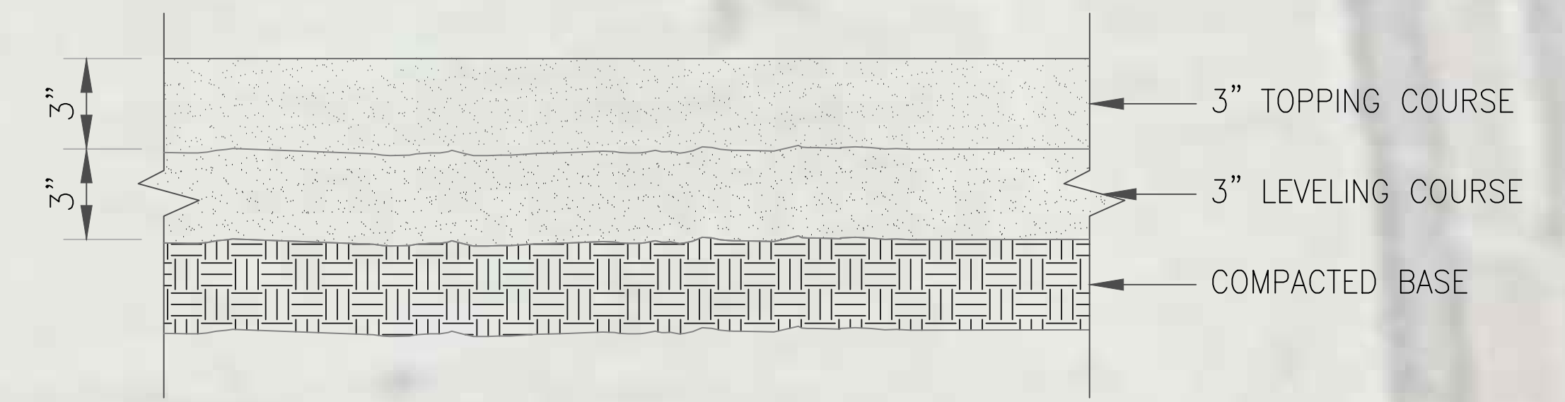
1 TYPICAL ASPHALT SECTION
