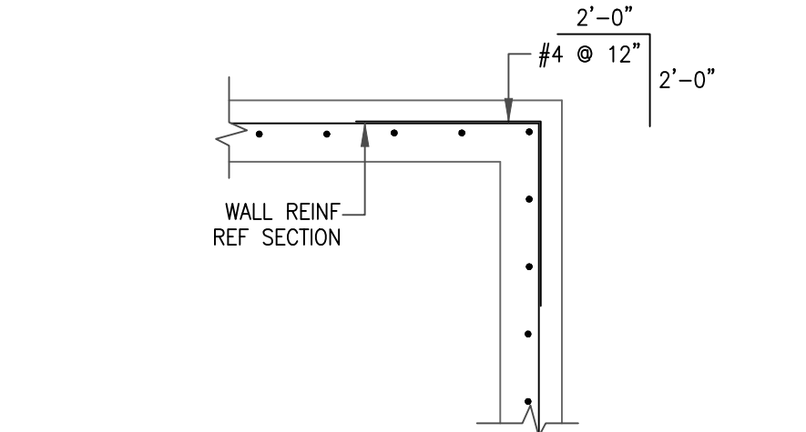
10 TYP. WALL INTERSECTION/CORNER
