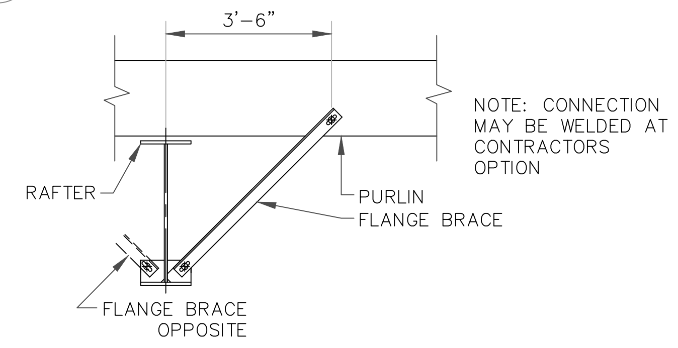
5 TYPICAL FLANGE BRACE @ PURLIN
