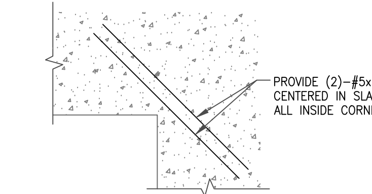
6 TYP SLAB ON GRADE REINFORCING
