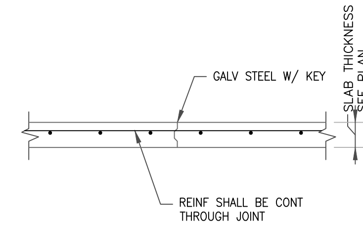
3 TYP SLAB CONSTRUCTION JOINT
