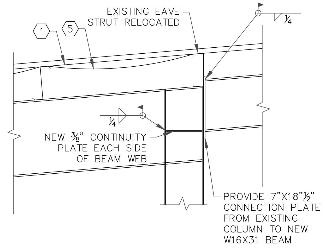
1 CONNECTION TO EXISTING STRUCTURE
