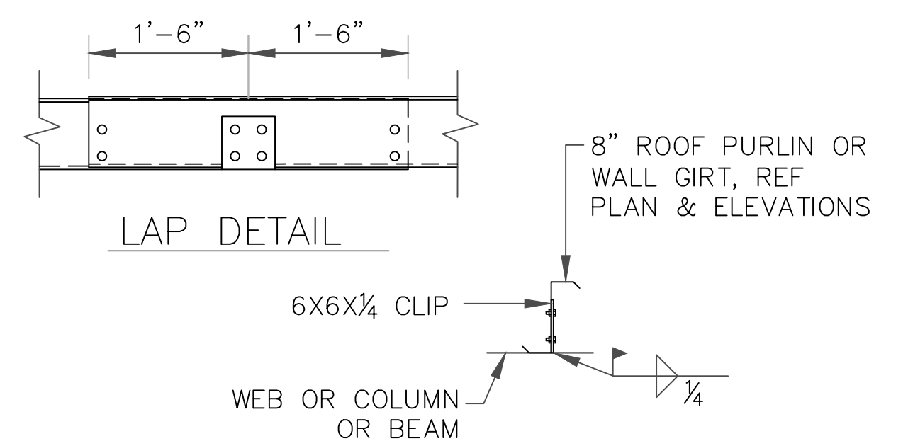
3 WALL GIRT AND ROOF PURLIN CONNECTION DETAIL
