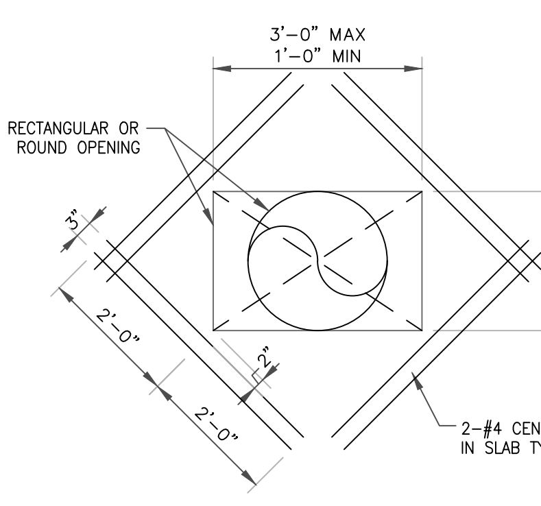
8 TYP OPENING IN SLAB ON GRADE
