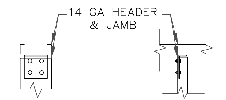
6 TYPICAL HEADER & JAMB DETAIL
